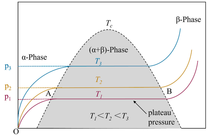
Fig. 2. Diagram of P-C-T curve of MH absorption/desorption of hydrogen.
